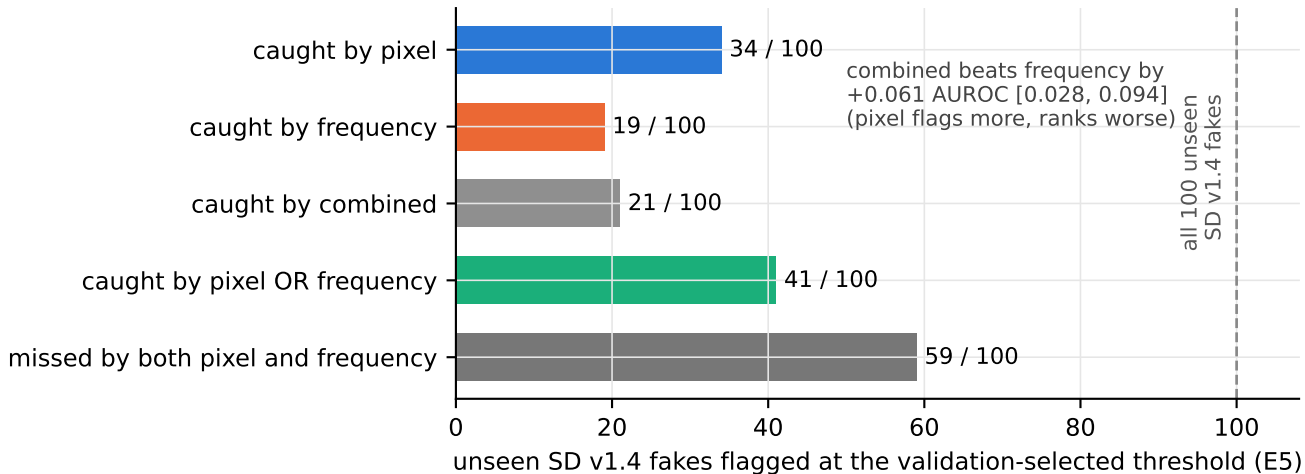
The two arms catch different fakes (E5, unseen SD v1.4)
