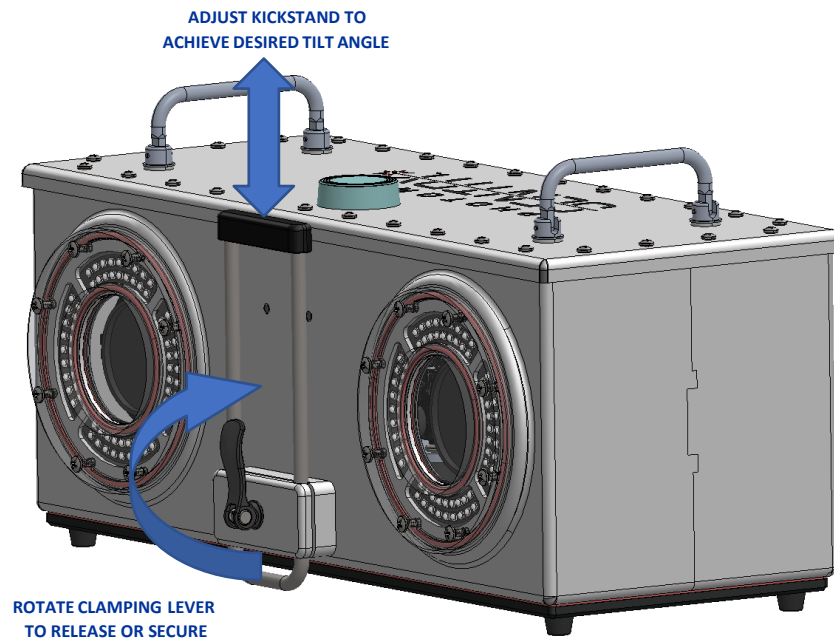
Figure 3: Tilt mechanism
