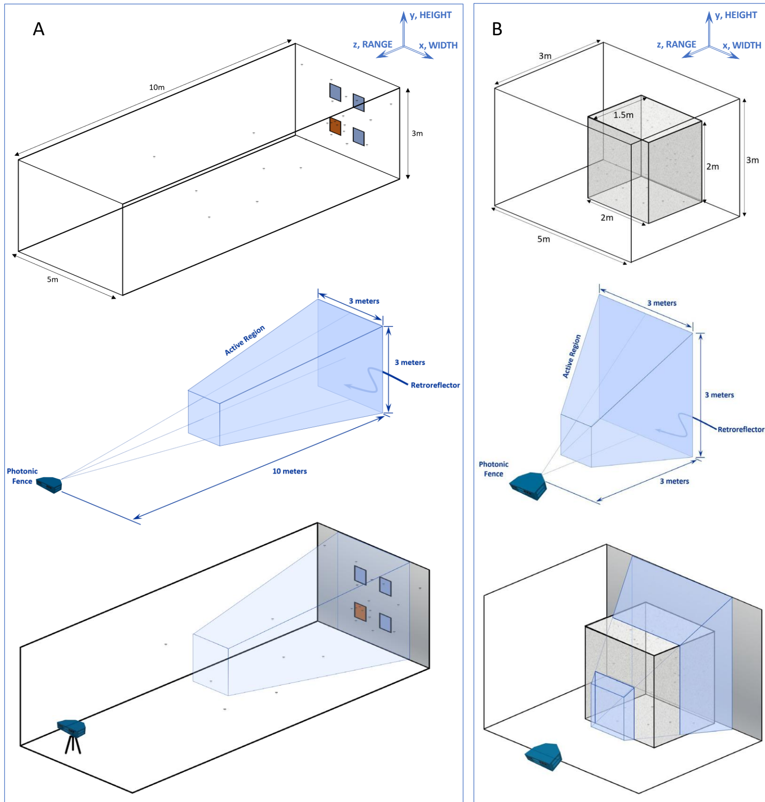
Figure A10: Reference Photonic Fence Monitoring Device Installations: A – LAB configuration, B – MINI configuration
