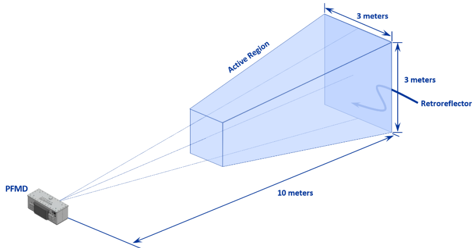
Figure 1: Representative PFMD configuration
