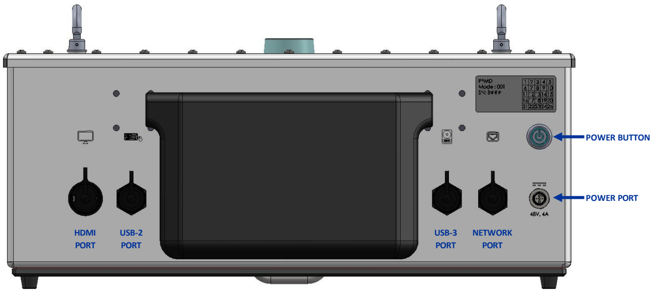
Figure 2: PFMD rear panel features
