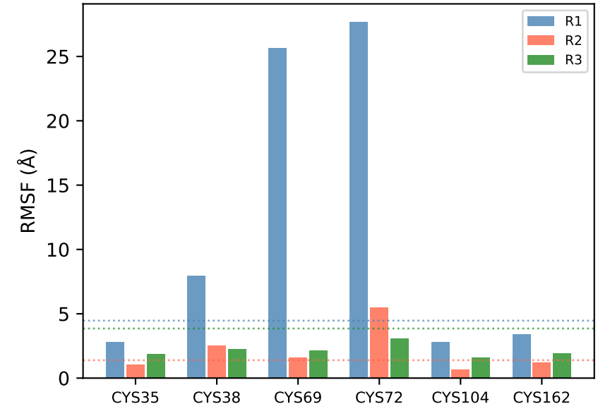
CxxC Motif RMSF (nokta = global ort)
