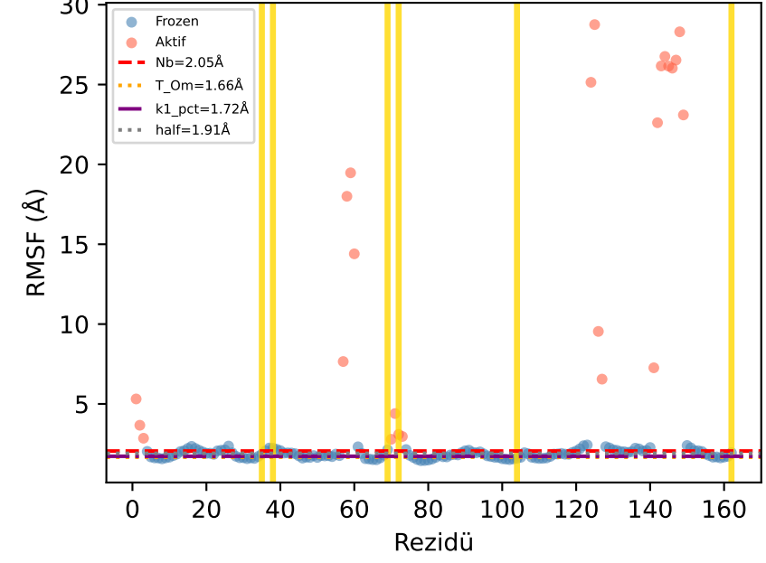
R3 | ort=3.853Å Aktif=0.1481 CxxC/g=0.556
