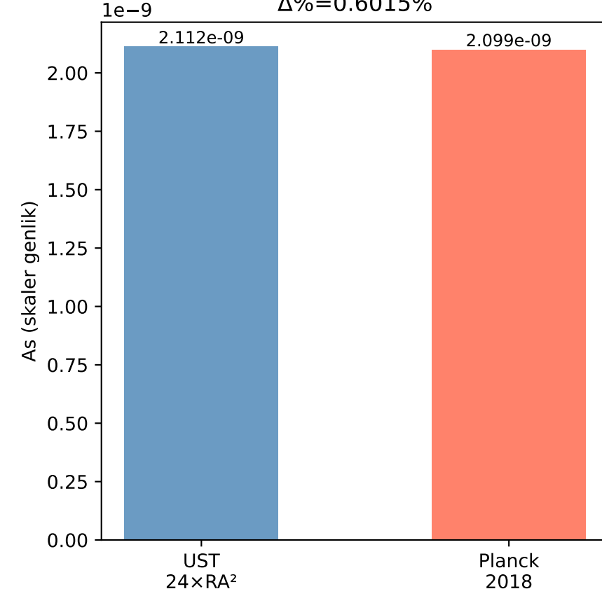
CMB Skaler Genliği 24×RA 2 vs Planck 2018 Δ%=0.6015%
