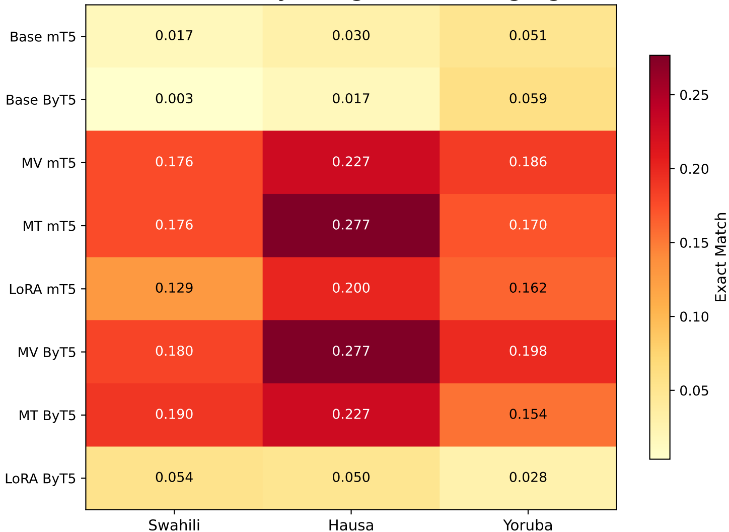
Exact Match by Configuration × Language
