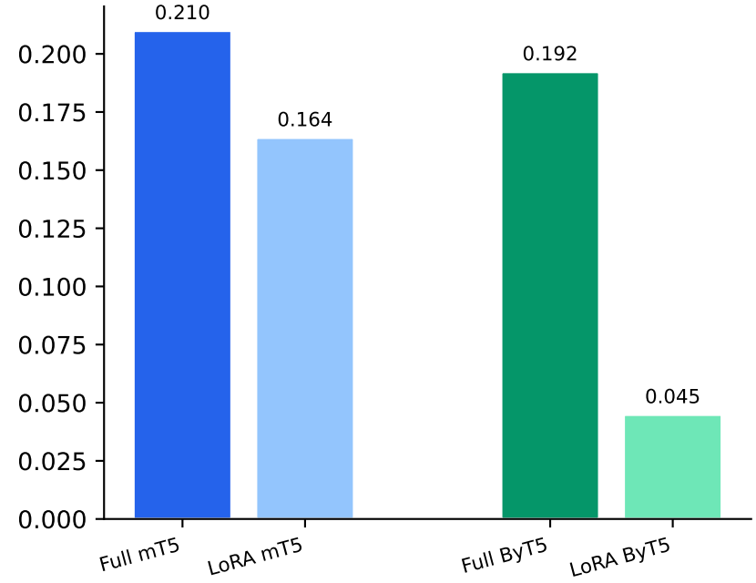
Exact Match
