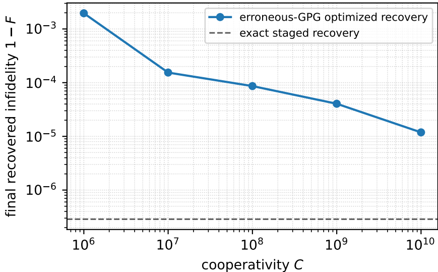
Noisy GPG sweep at p = 1e - 03
