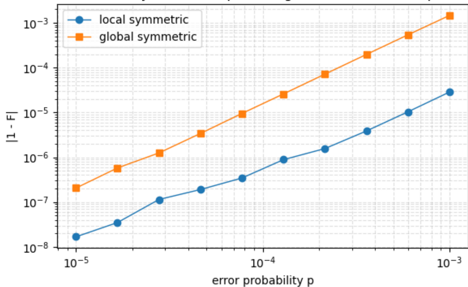
Global vs local symmetric depolarizing noise on Gross 13-qubit code
