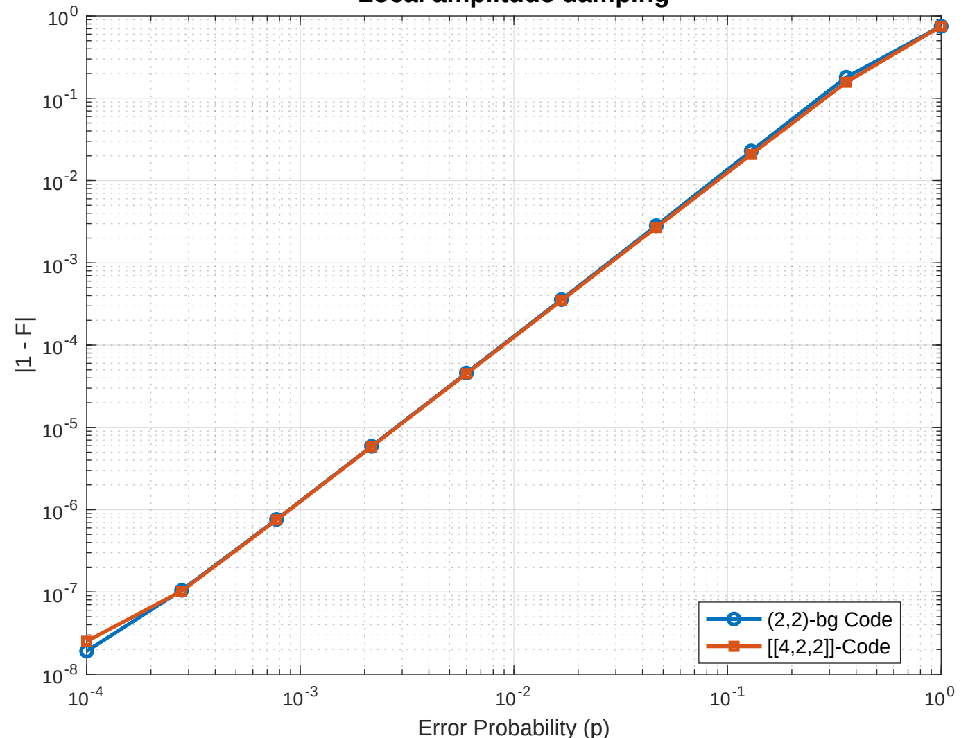
Local amplitude damping
