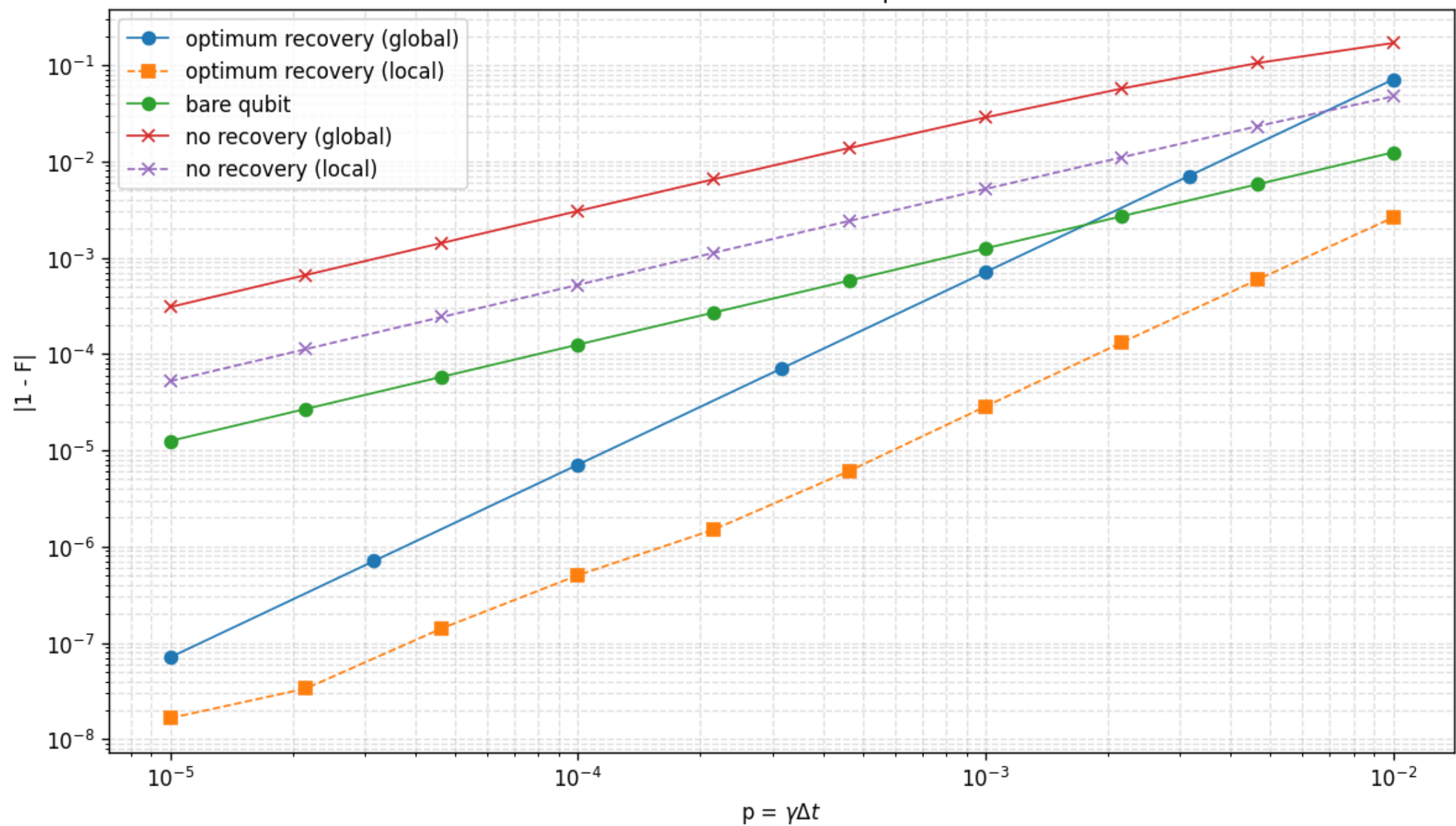
Performance of Gross 13-qubit code
