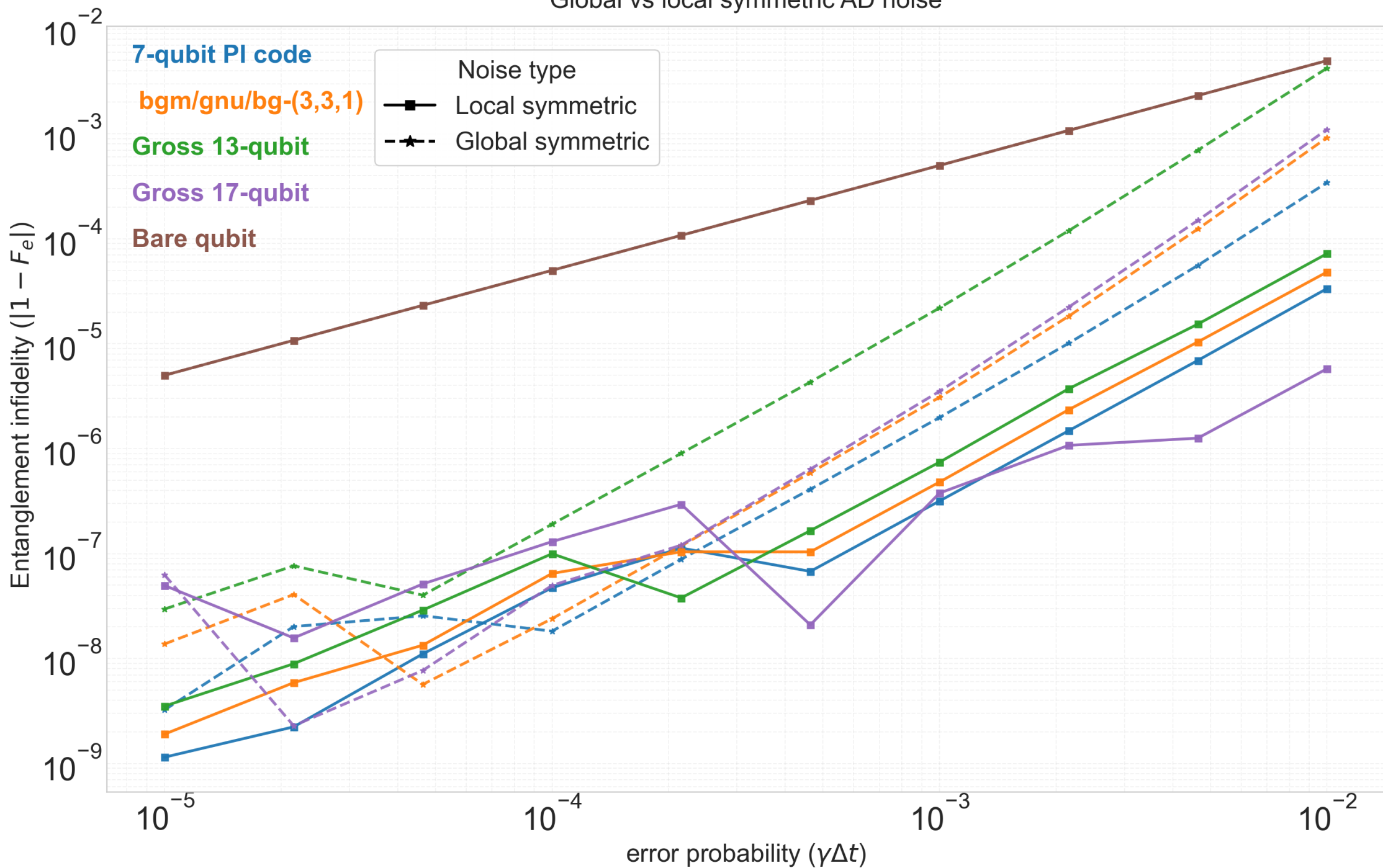
Global vs local symmetric AD noise
