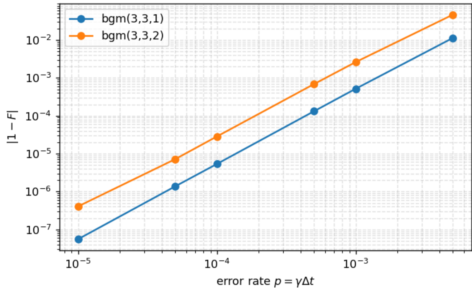
Global symmetric depolarising
