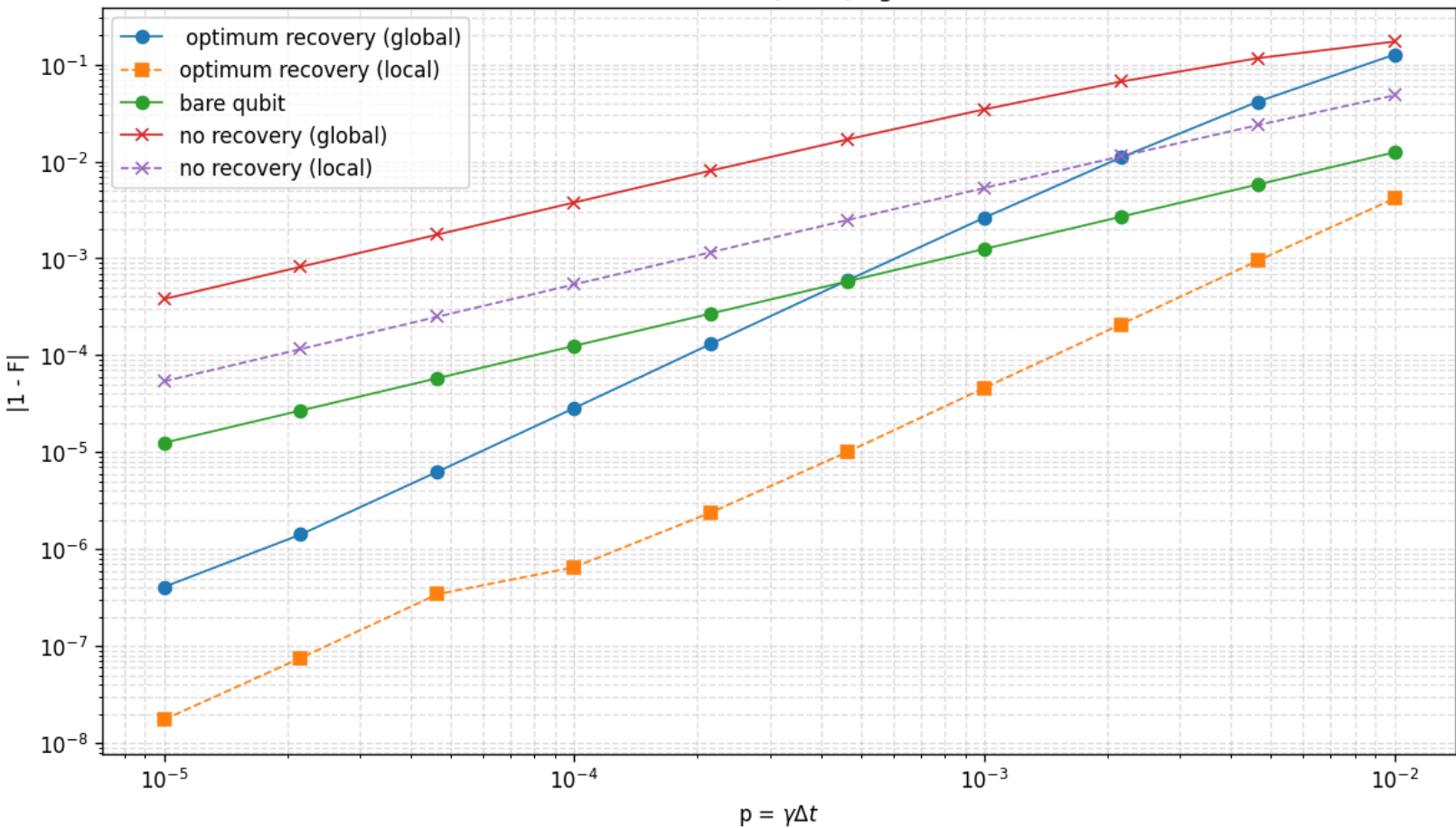
Performance of (3,3,2) bgm code
