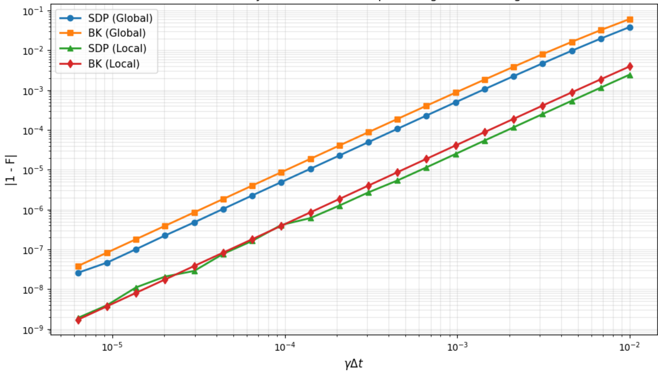
SDP vs BK Recovery: Global &amp; Local Depolarizing for (3,3,1) bgm code
