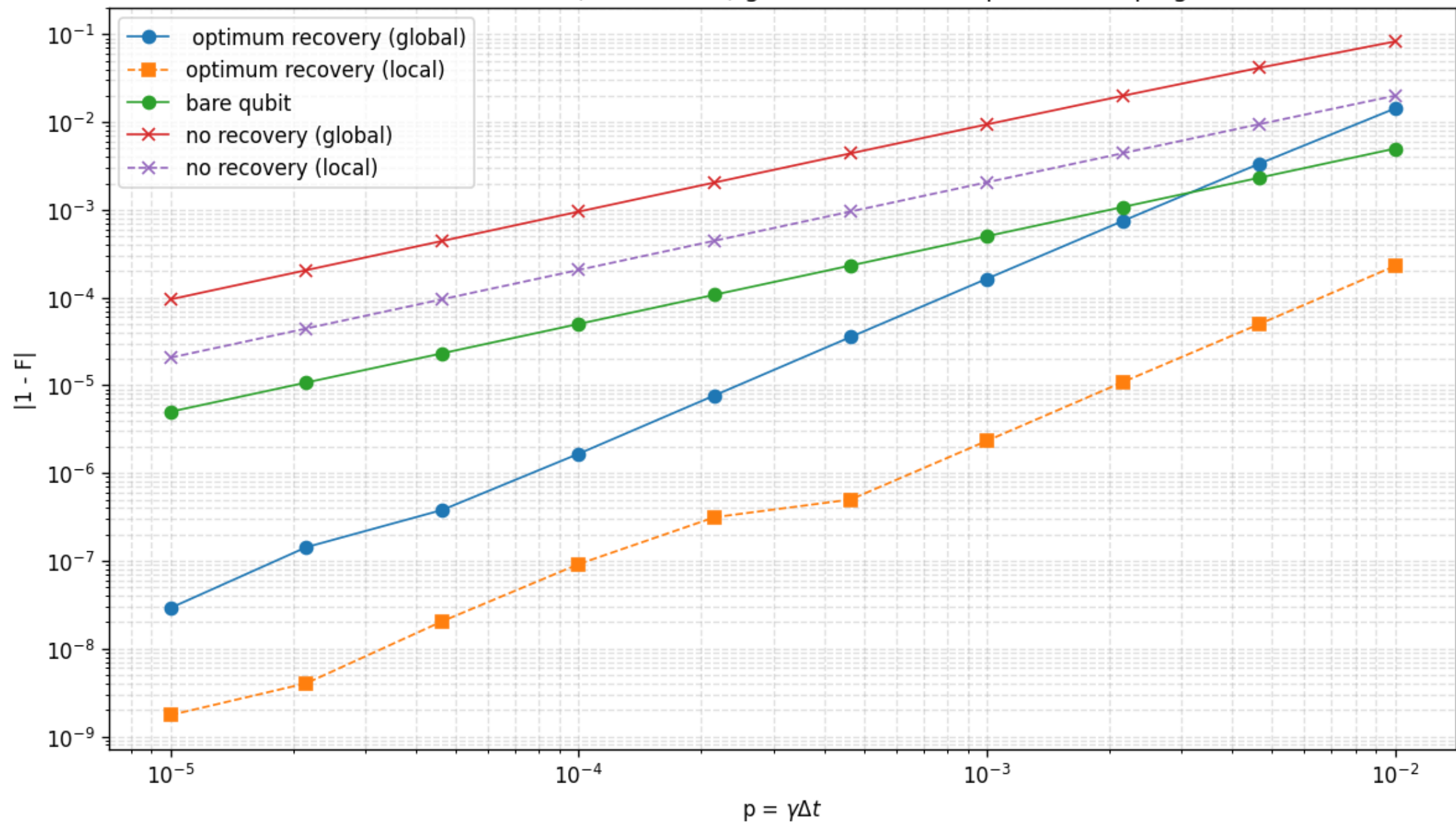
Performance of (2, 4, 1 + 1/8) gnu code under amplitude damping
