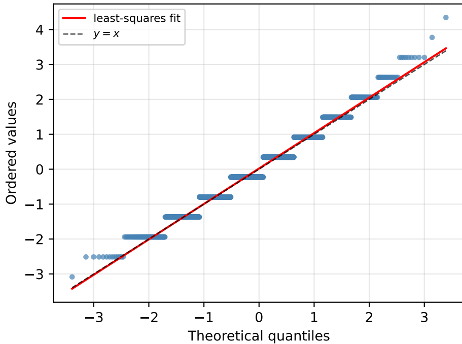
QQ vs N(0, 1) ( \Lambda = 2 )
