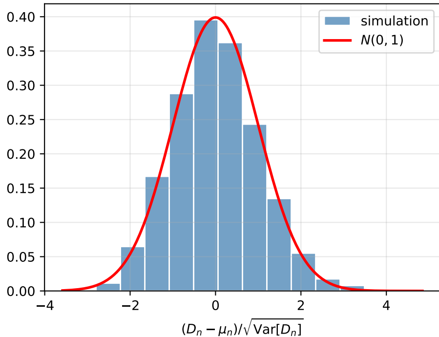
Studentized histogram ( \Lambda = 2 , n = 5000 )
