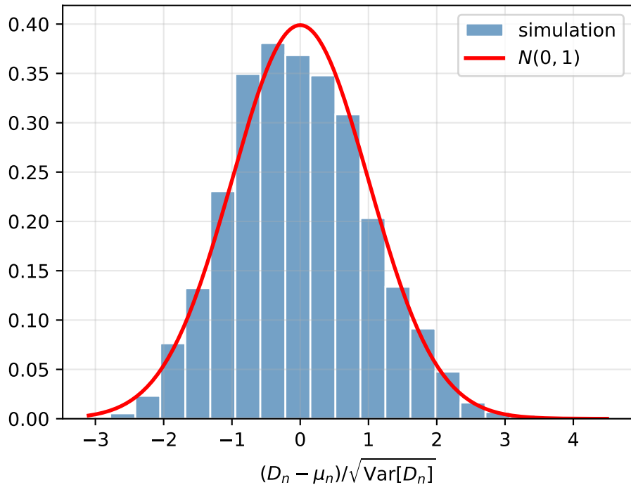
Studentized histogram ( \Lambda = 1, n = 5000 )
