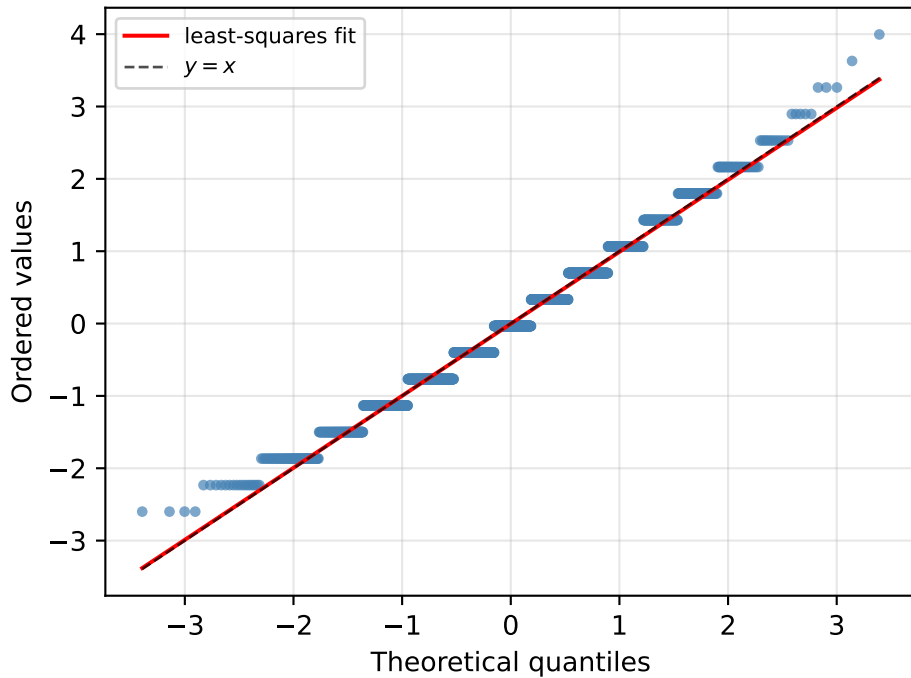
QQ vs N(0, 1) ( \Lambda = 1 )
