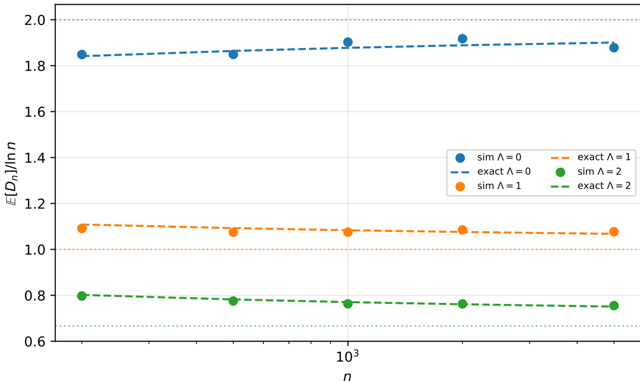
Finite- n mean ratio (dotted = asymptotic limit 2/(1 + \Lambda) )
