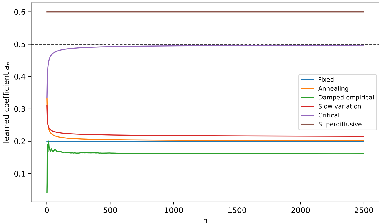
Representative learned-memory trajectories
