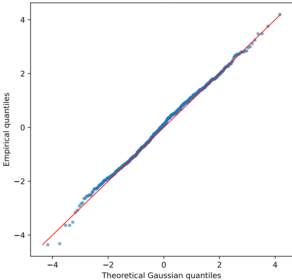
LC-ERW QQ plot: fixed
