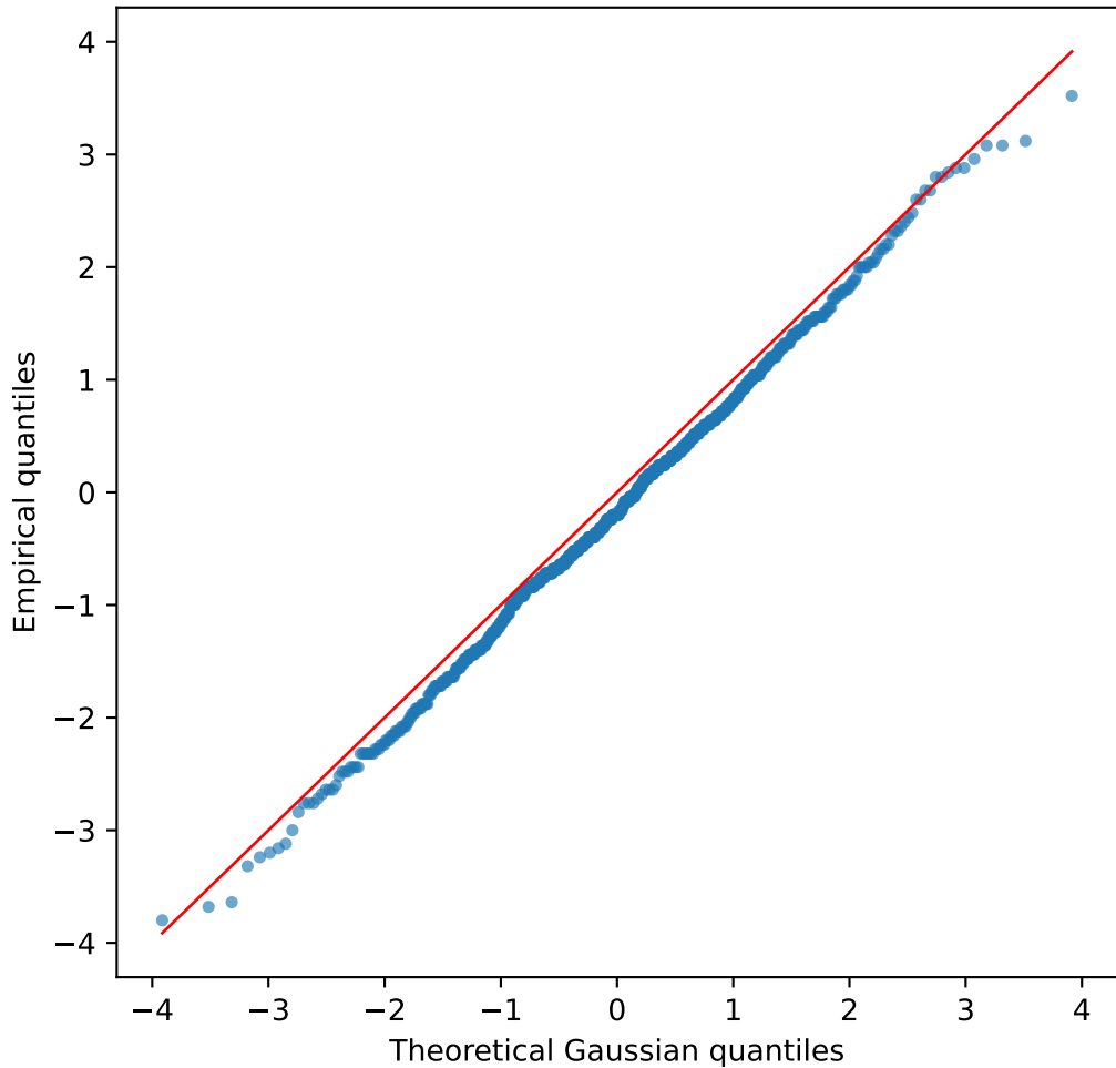
LC-ERW QQ plot: damped_empirical
