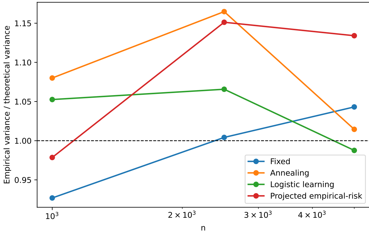
Variance-ratio convergence across sample sizes
