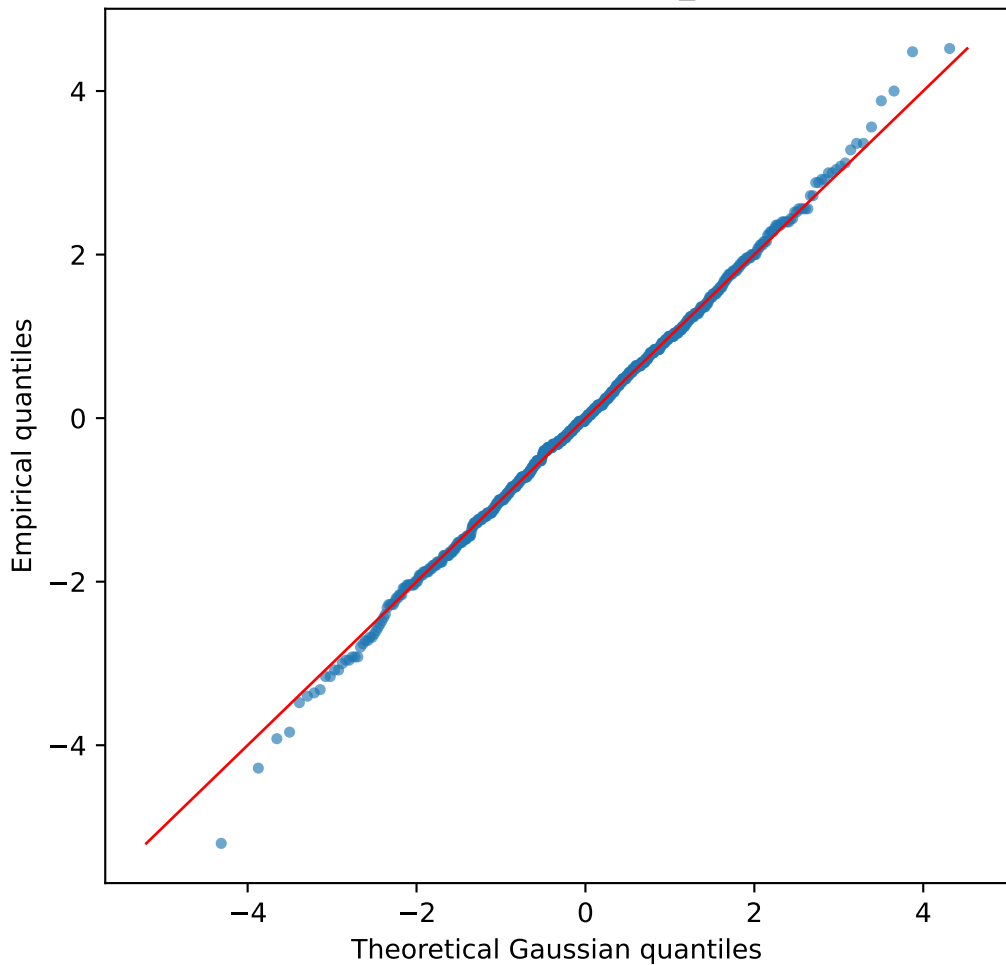
LC-ERW QQ plot: logistic_learning
