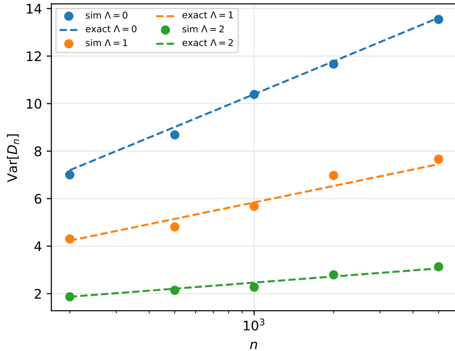
Variance (exact formulae)
