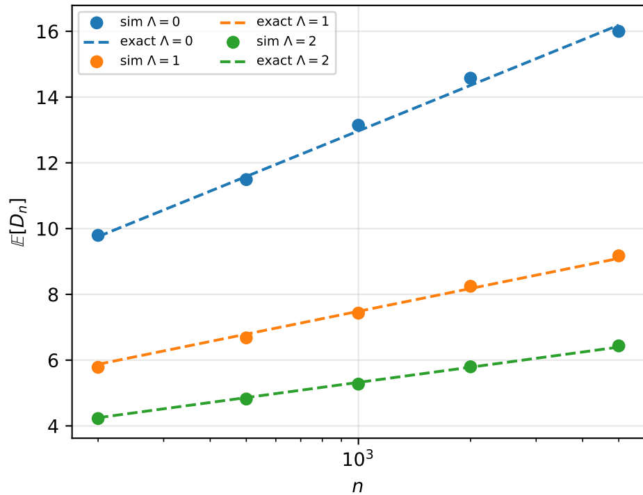
Mean depth (exact formulae)
