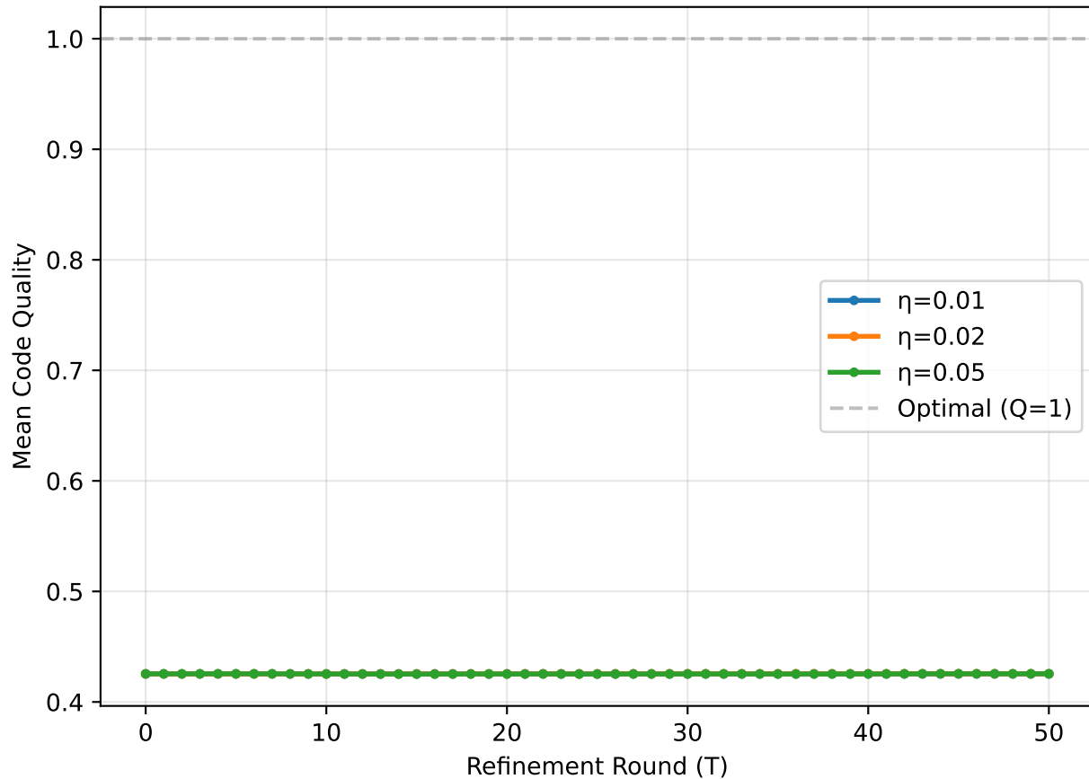
Quality vs. Rounds (diversity=0.5)
