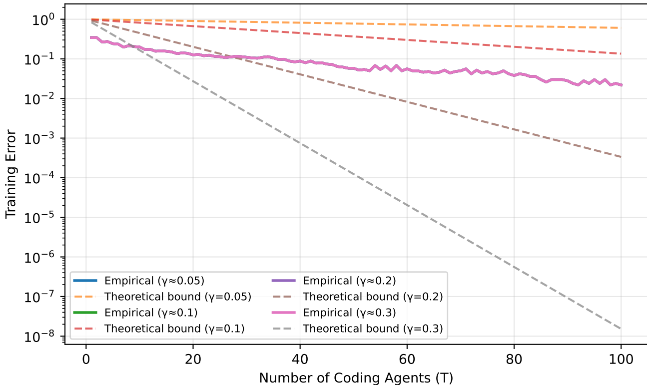
Training Error vs. Number of Weak Coding Agents
