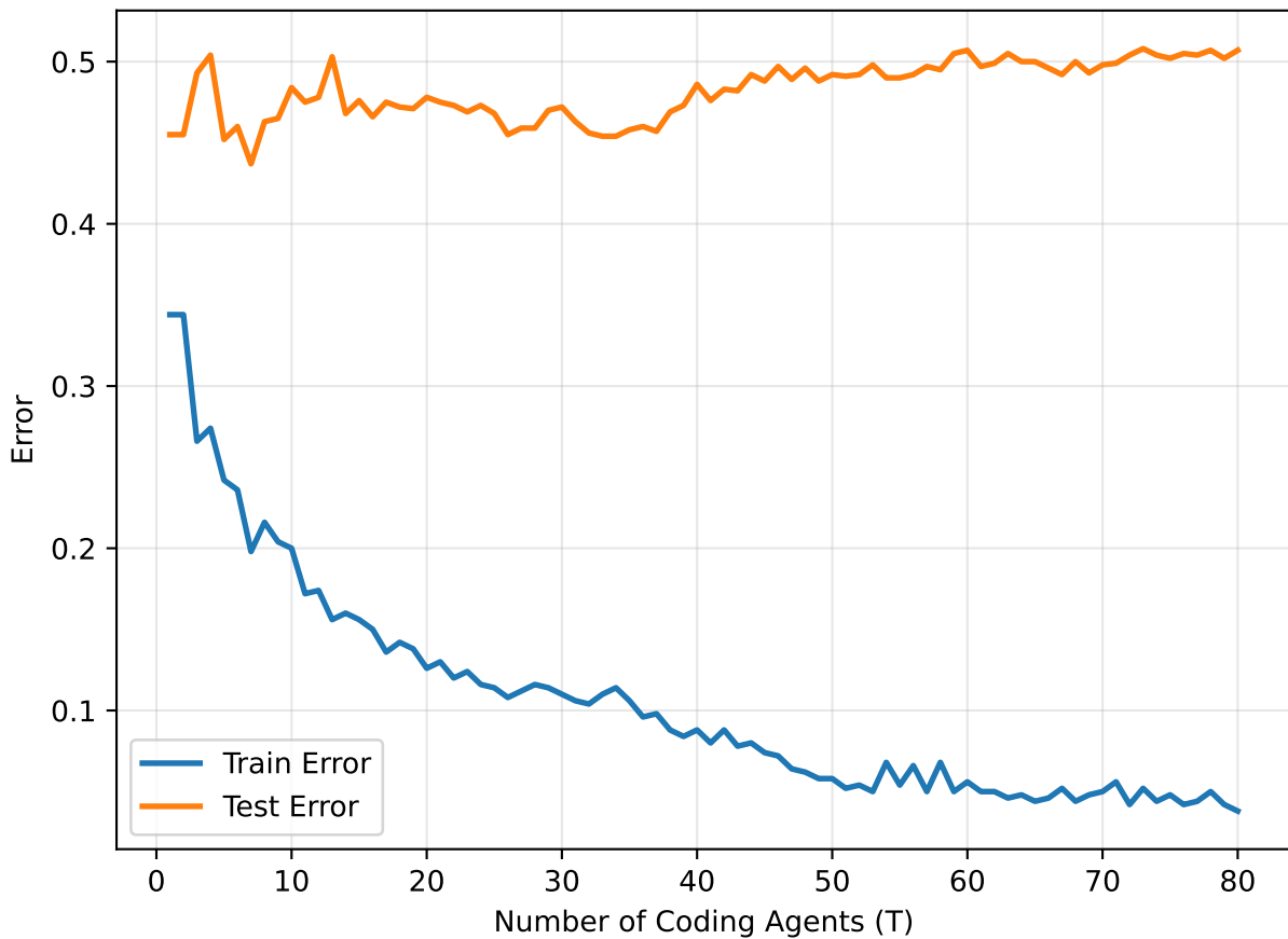
Train vs. Test Error (N=500)
