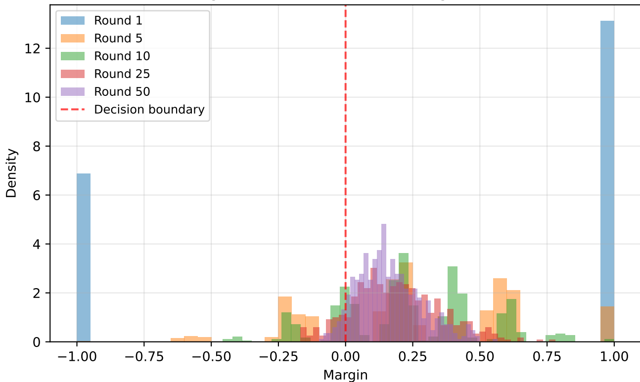
Margin Distribution Over Boosting Rounds
