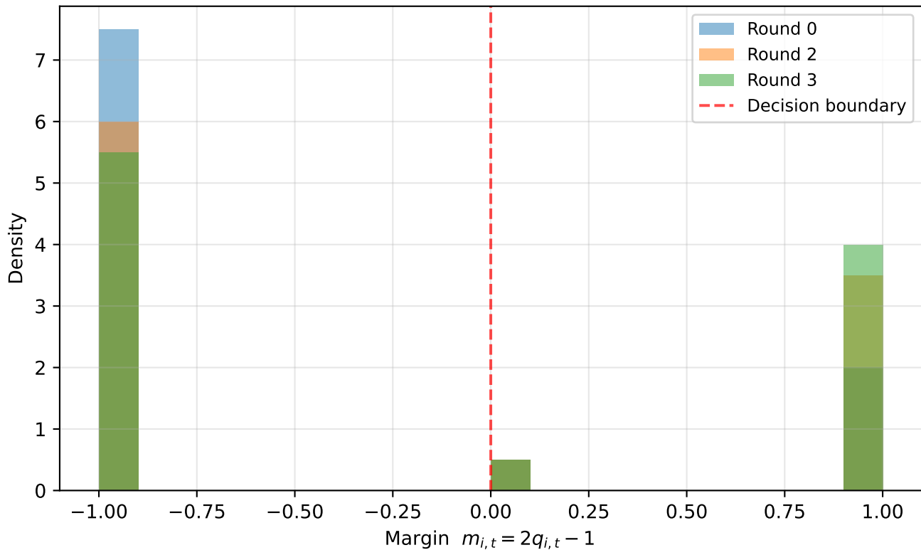
LLM Refinement: Margin Distribution Over Rounds
