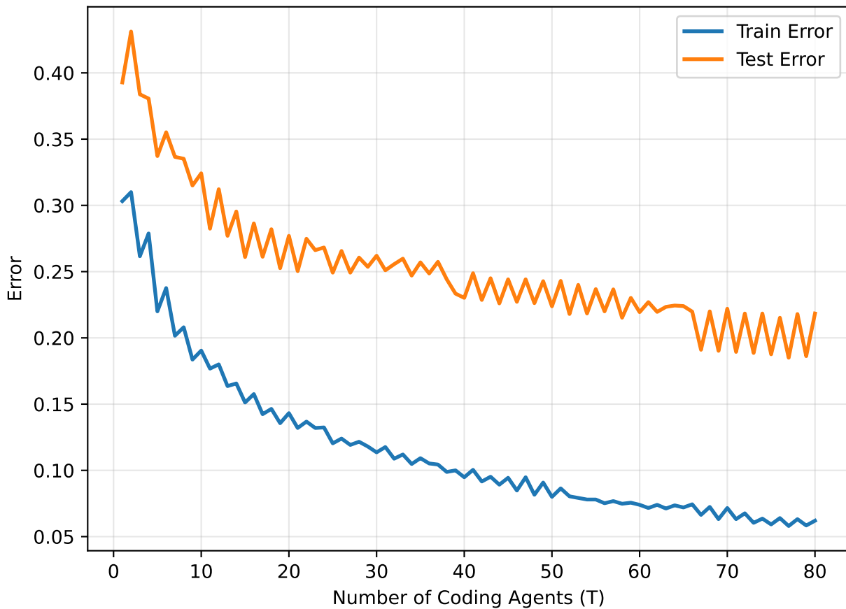
Train vs. Test Error (N=500, SWE-bench)
