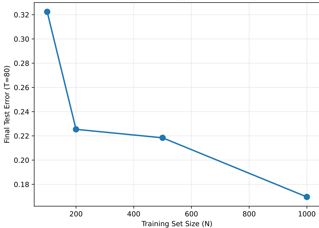
Generalization vs. Sample Size (SWE-bench)
