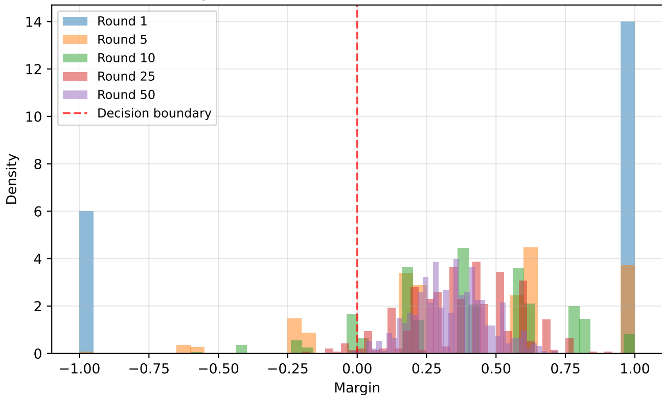
Margin Distribution Over Rounds (SWE-bench)
