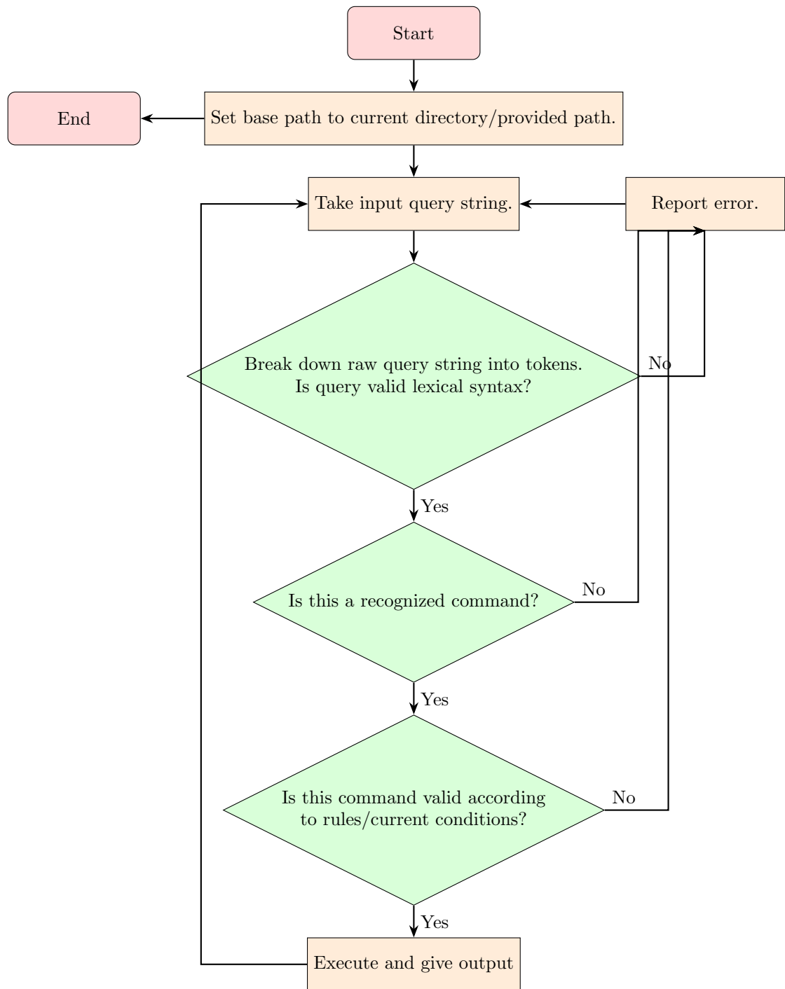
Figure 3: Compiler Operation Loop
