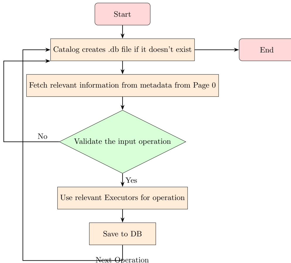
Figure 2: Catalog Operation Loop
