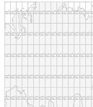
Asia | Local 0/240 fitted
