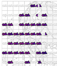
Europe | Local 105/210 fitted
