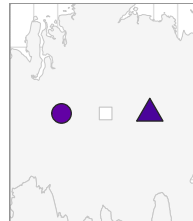
Asia | Continental 2/3 fitted
