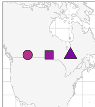
America | Continental 3/3 fitted
