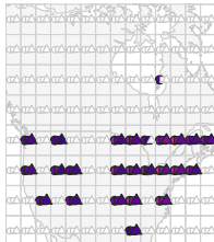
America | Local 72/336 fitted
