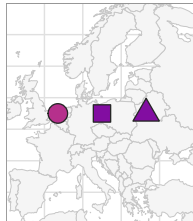
Europe | Continental 3/3 fitted
