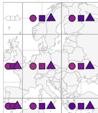
Europe | Regional 24/27 fitted
