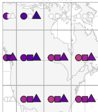
America | Regional 24/36 fitted
