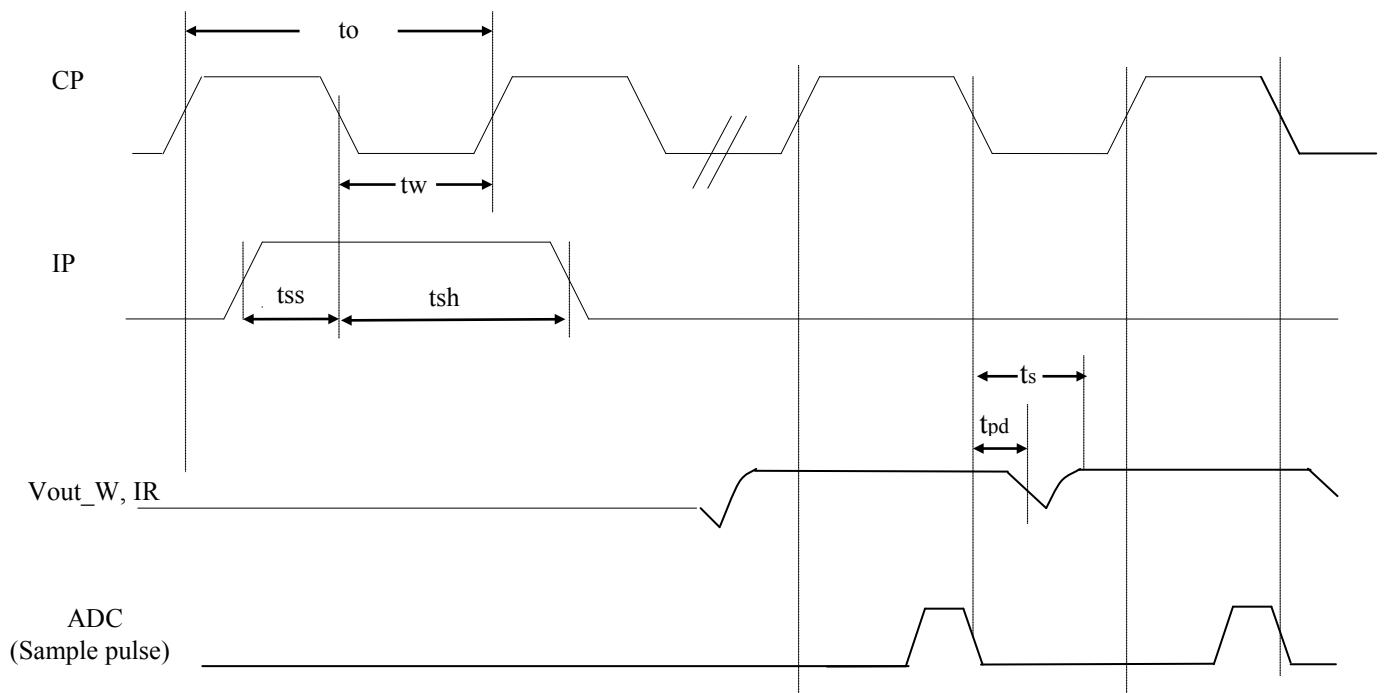
Figure 4. Switching Waveforms
