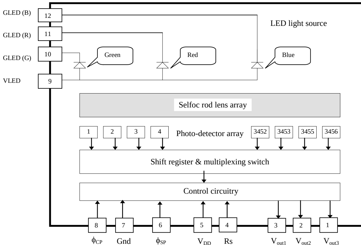
Figure 2. M118-232C3 color CIS module block diagram.
