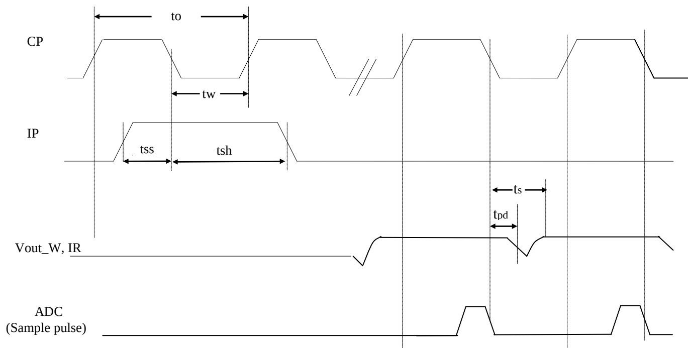
Figure 4. Switching Waveforms
