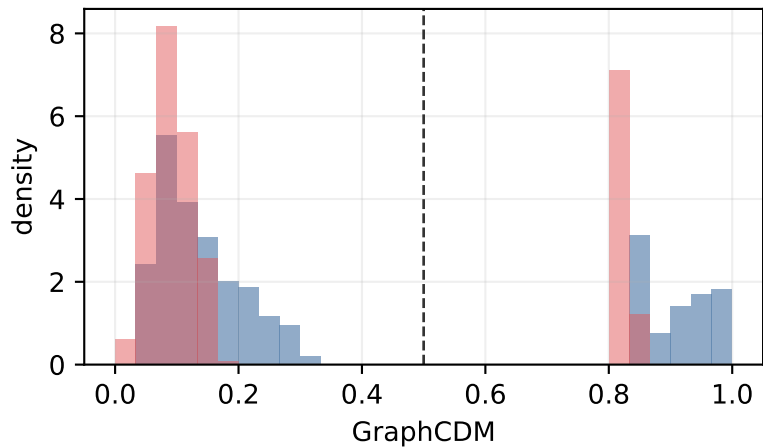
UNSW-NB15, tail asym 40%
