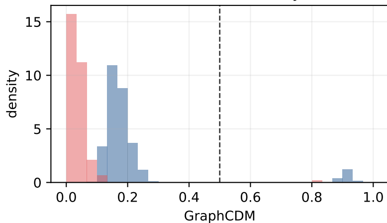
UNSW-NB15, tail asym 60%
