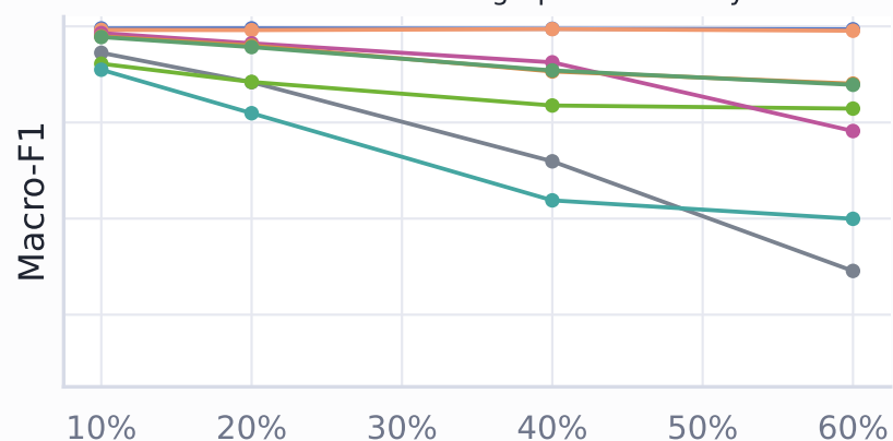
UNSW-NB15: graph-consistency
