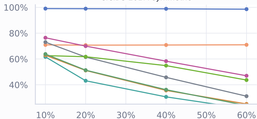
CESNET-TLS-year22: symmetric
