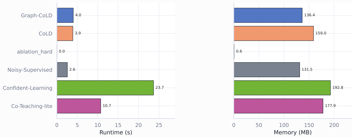
Figure 5: Runtime and memory cost by method.
