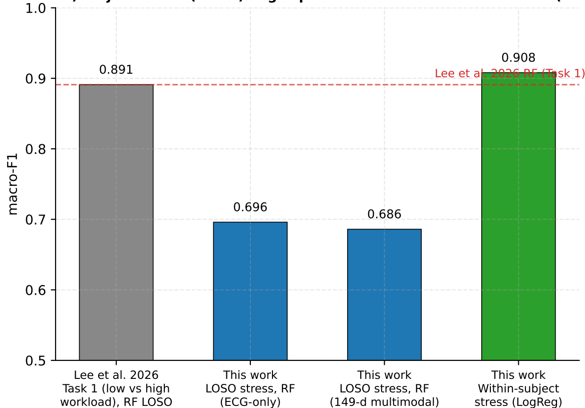
B. Stress / workload binary classification on EmoWork (matched metric)
