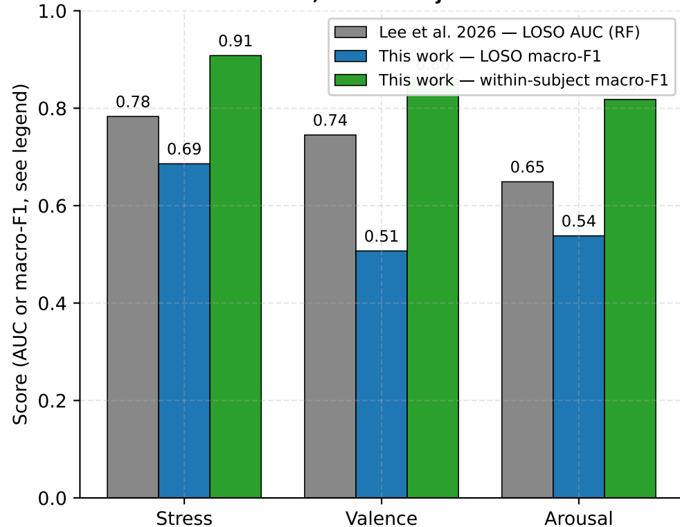
A. EmoWork dimensional targets vs Lee et al. 2026
