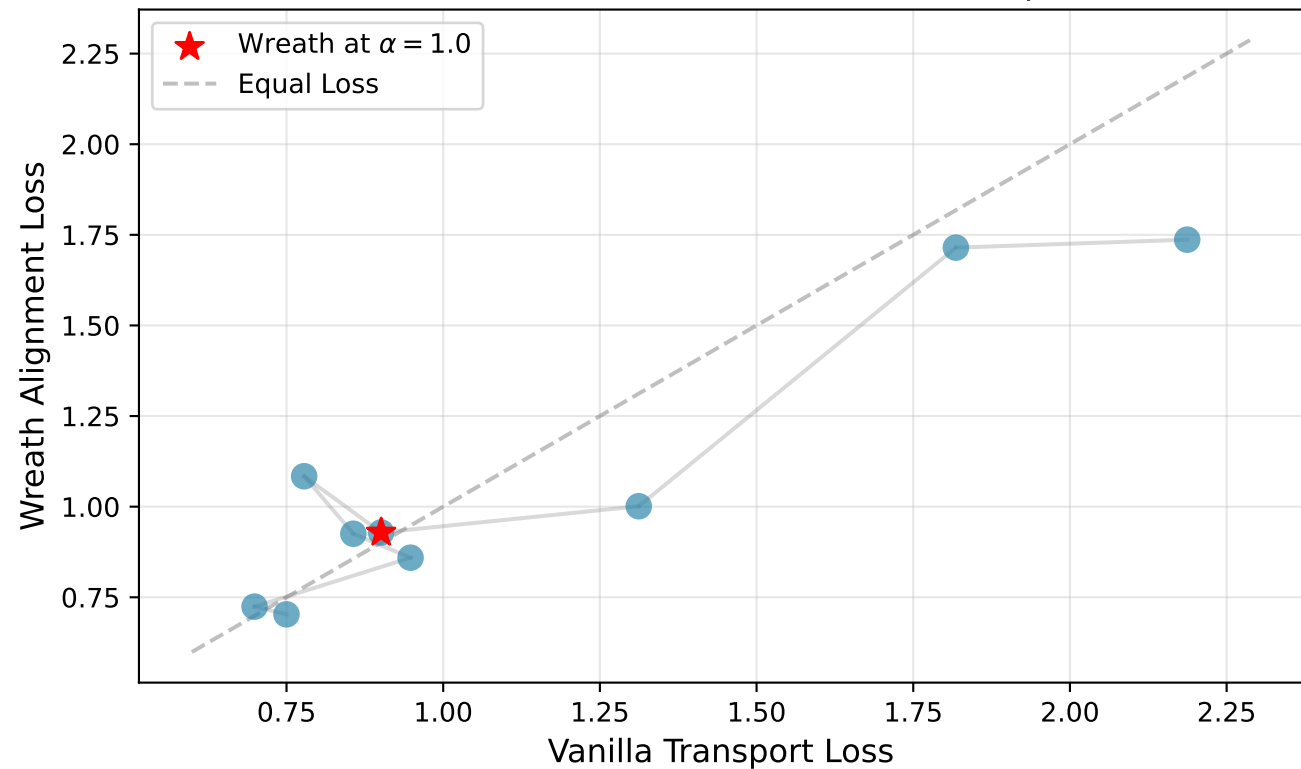
Wreath vs. Vanilla: Task Loss Landscape
