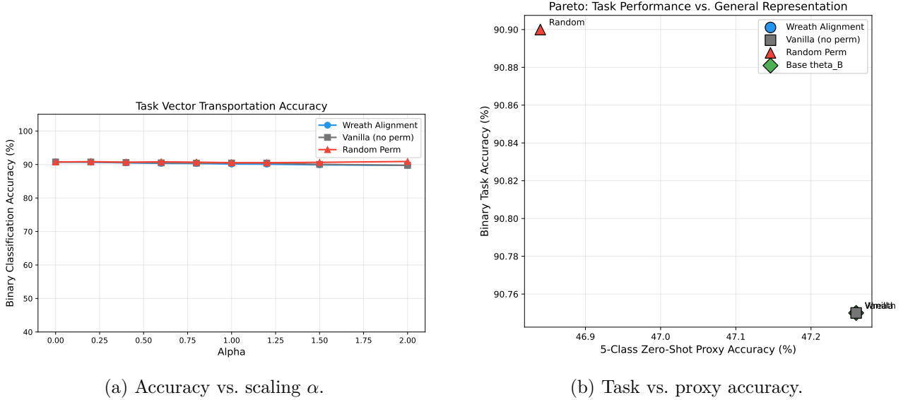
Figure 3: Exp. 3: Small-scale proof-of-concept task vector transport. Note the narrow y -axis range in (b); differences are within sampling noise.
