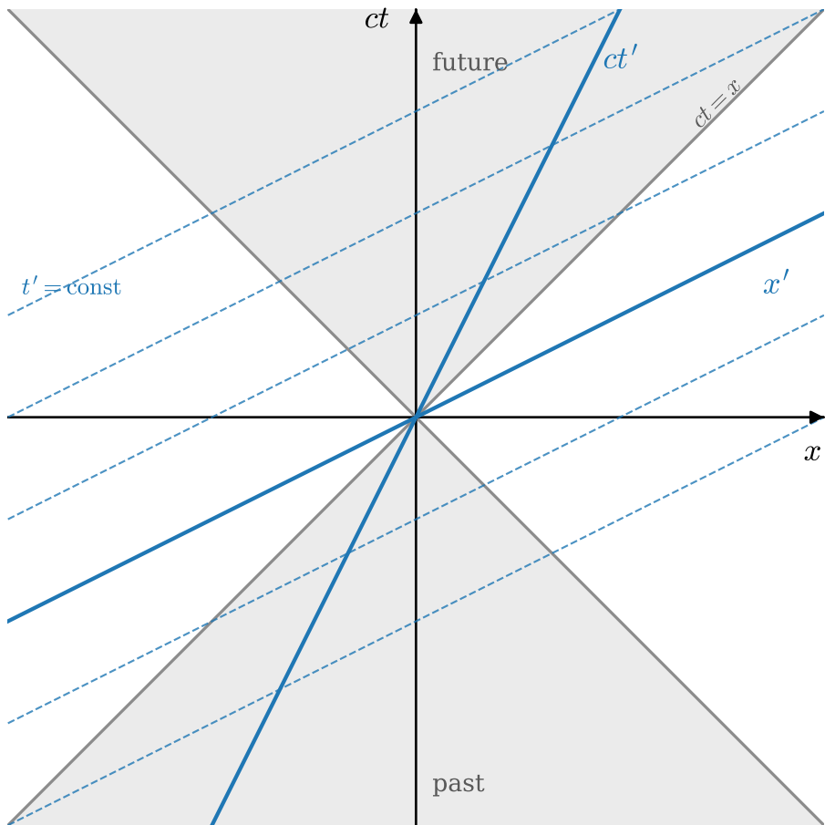
Boosted axes and simultaneity slices, \beta = 0.5
