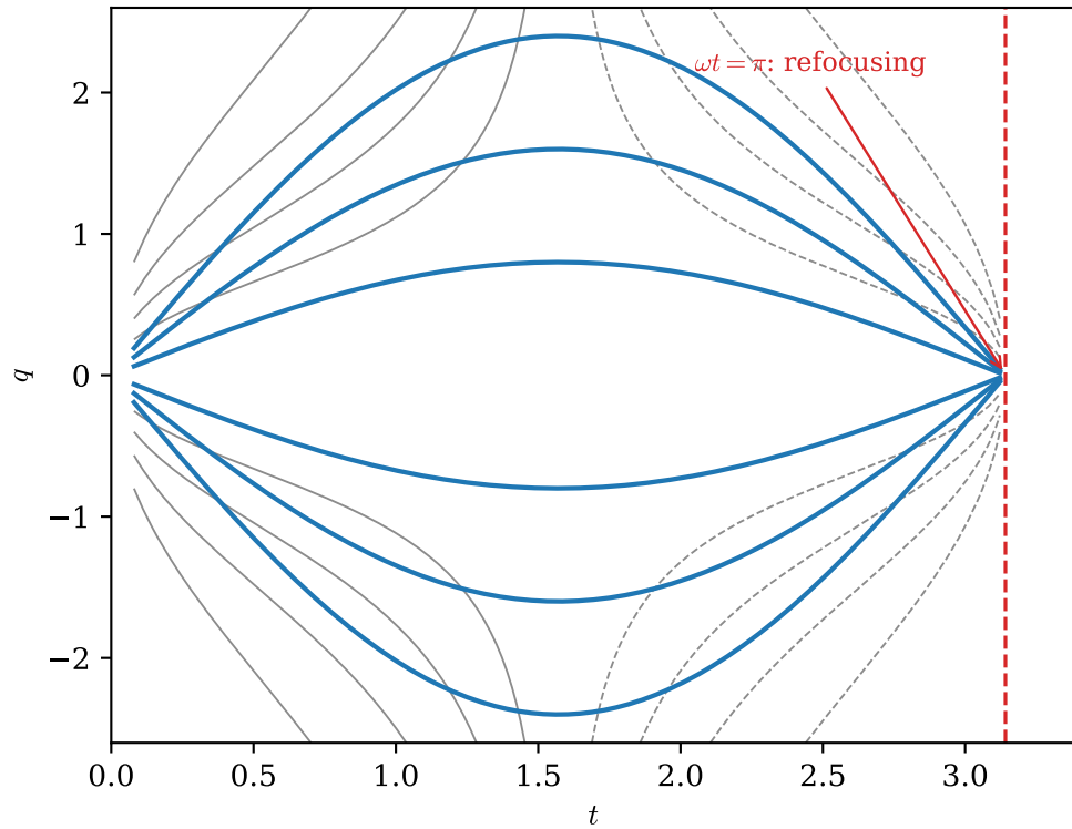
oscillator: S = (q^2/2)\cot t
