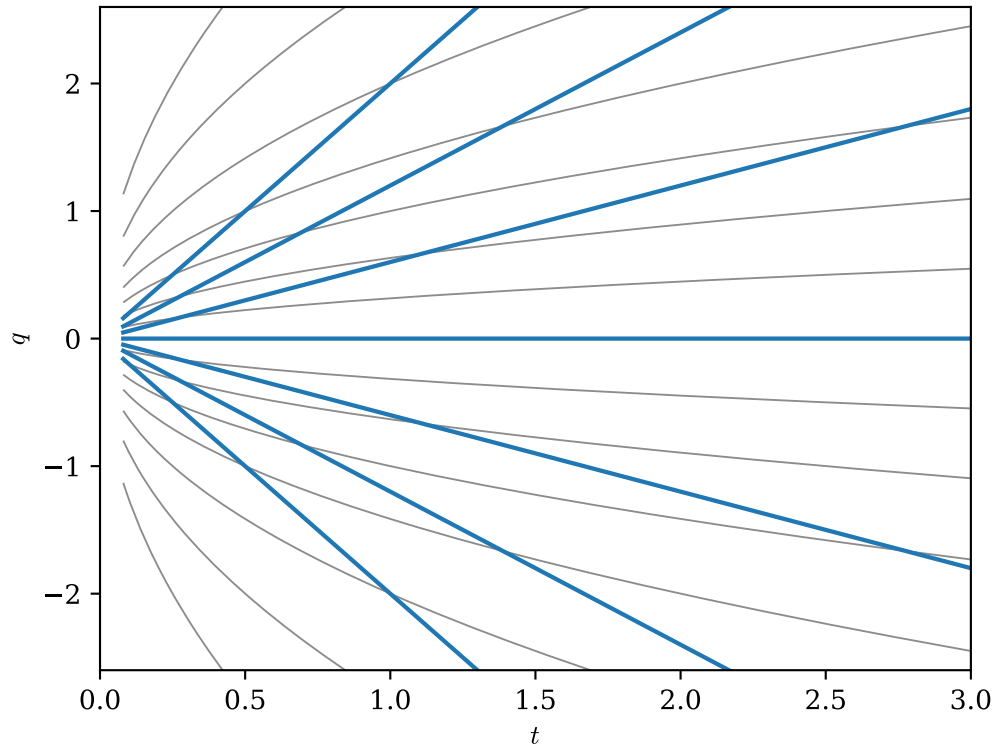
free particle: S = q^2/2t
