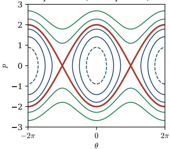
pendulum (red: separatrix)
