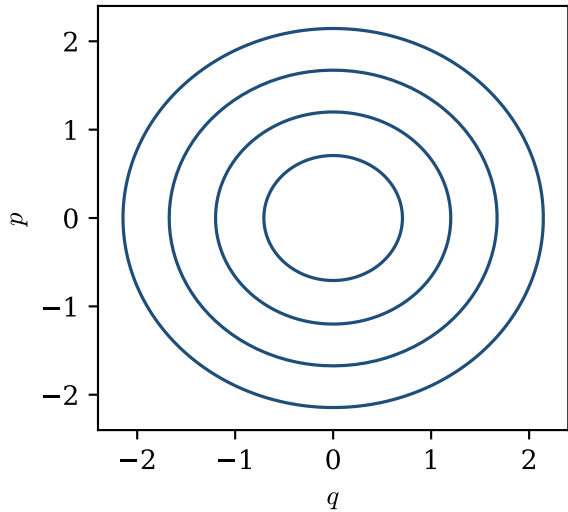
harmonic oscillator
