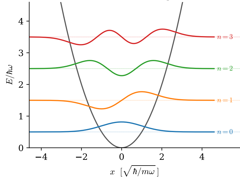
u_n at their levels in V = \frac{1}{2}m\omega^2 x^2
