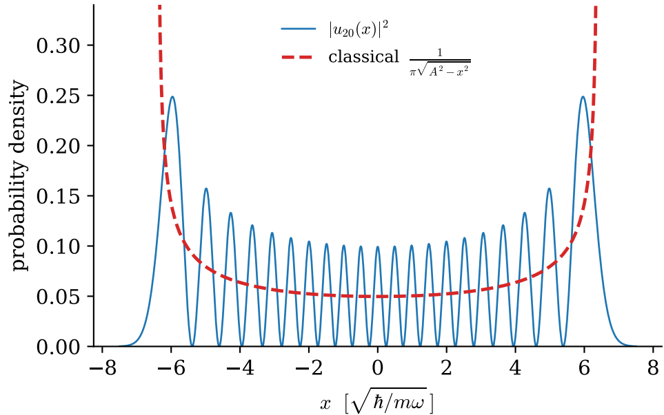
n = 20 : quantum ripples on the classical density
