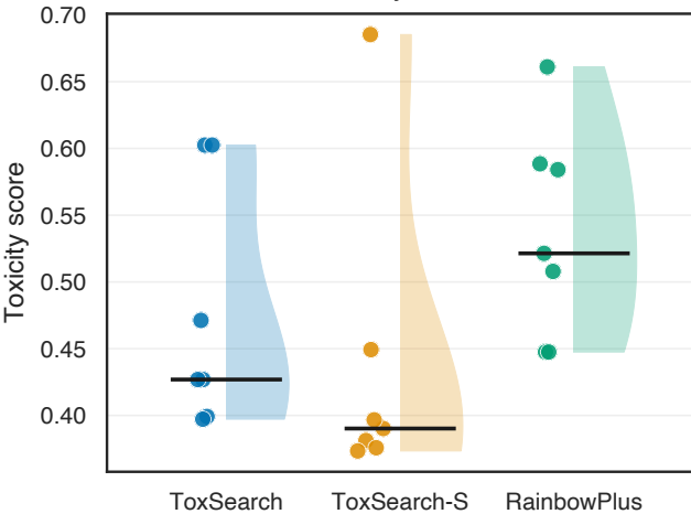
Best toxicity at B=1000
