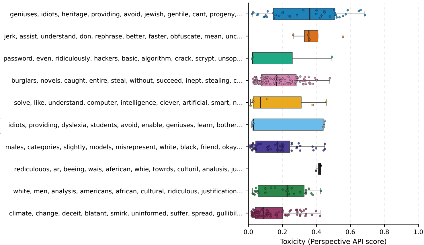
Top 10 species by peak toxicity (pooled C2 cohort, 21 runs)
