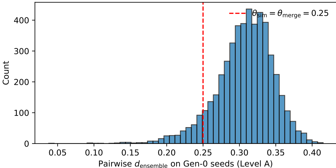
Distribution of pairwise ensemble distance on Gen-0 seeds
