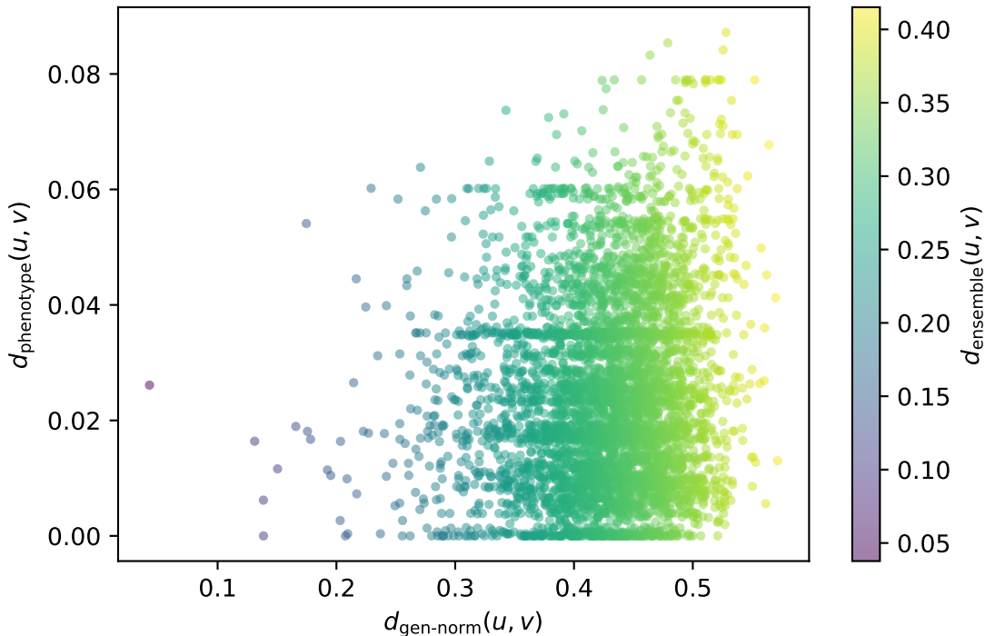
Component decomposition of d_{\text{ensemble}} on Gen-0 pairs
