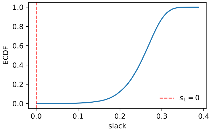
Triangle slack s_1 (tight, all triples)
