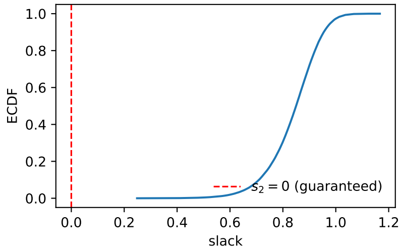
2-inframetric slack s_2 (tight, all triples)
